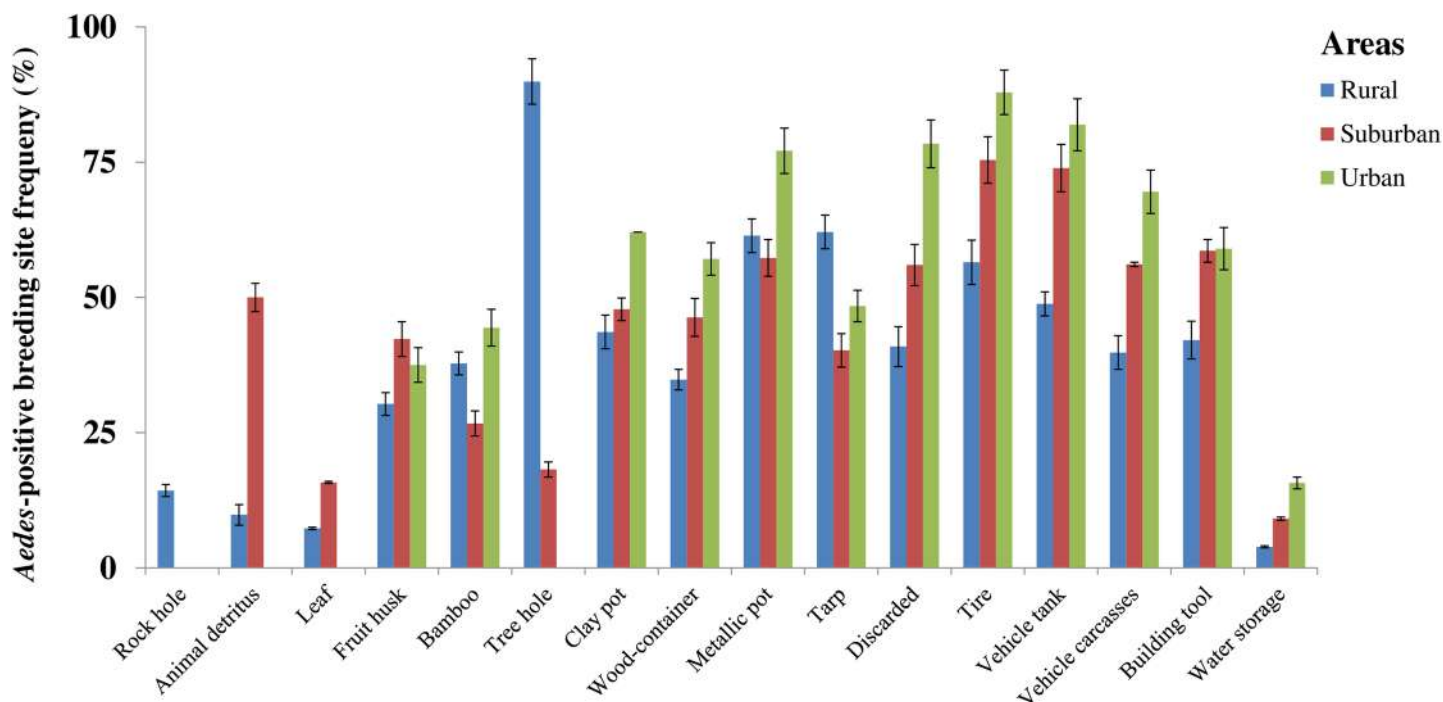
Fig 2. Dynamics of Aedes mosquito breeding sites in rural, suburban, and urban areas in south-eastern Côte d'Ivoire from January 2013 to October 2014. Error bars show the standard error (SE).
